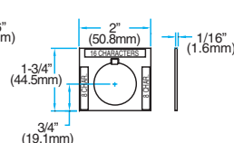
LP-40-SP SHORT
