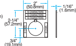
LP-40-SP TALL
