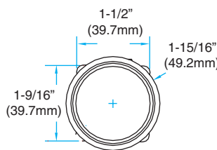
ILLUMINATED SHROUDED MUSHROOM LENS (SIPBC)
