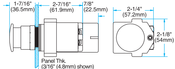
ILLUMINATED TRANSFORMER AND RESISTOR OPERATORS (SHOWN WITH IMC)
