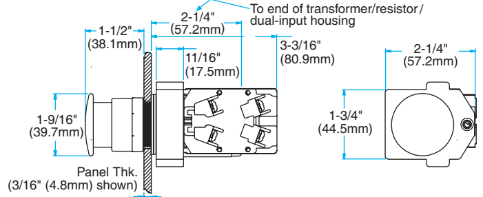
ILLUMINATED SHROUDED MUSHROOM LENS (SIPBC)
