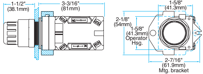
TRANSFORMER & RESISTOR PUSH-TO-TEST OPERATORS (SHOWN WITH HIPBC)
