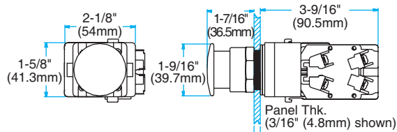
ILLUMINATED FULL VOLTAGE OPERATOR (SHOWN WITH IMC)
