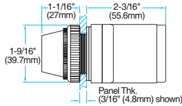
TRANSFORMER & RESISTOR PILOT LIGHT OPERATORS (SHOWN WITH PLL)
