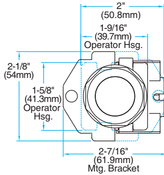
MAINTAINED FLUSH PUSH BUTTON CAP (SHOWN WITH AN OPERATOR AND CONTACT BLOCK)
