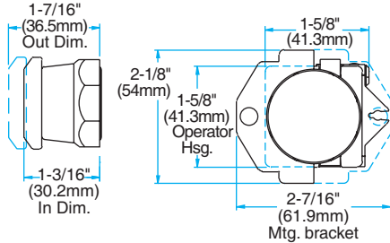
2-POSITION PUSH-PULL MAINTAINED 1-1/2" (38MM) MUSHROOM CAP
