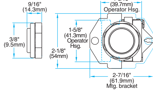
MOMENTARY EXTENDED CAP
