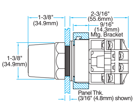
MAINTAINED FLUSH PUSH BUTTON CAP (SHOWN WITH AN OPERATOR AND CONTACT BLOCK)
