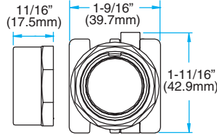
MOMENTARY GUARDED FLUSH CAP
