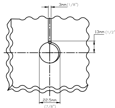
Drilling Plan
