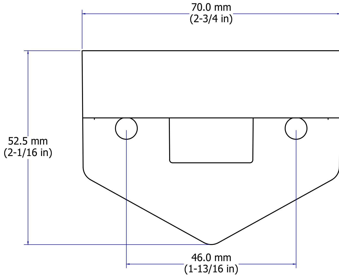
FRONT VIEW
