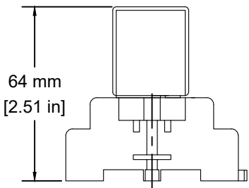
GPRM-B4C05 RELAY WITH GPRA-SB14U1 COMBINED HEIGHT SCALE 1:1
