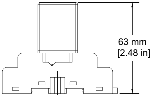
GPRM-B1C15 & B2C10 RELAY ASSEMBLED WITH GPRA-SB08G1 SOCKET
