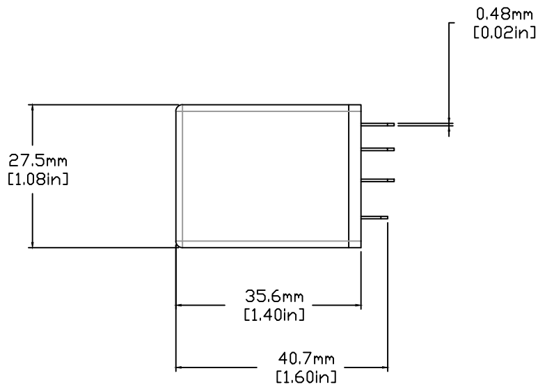
PLUG-IN TERMINAL
