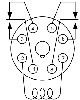
8 PIN DPDT
