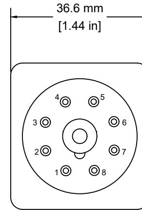
8 PIN OCTAL BASE
