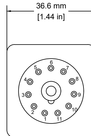
11 PIN OCTAL BASE
