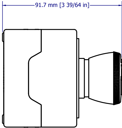
Single hole assembly w_PTR
