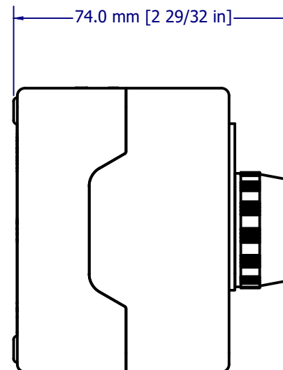
Single hole assembly w/pilot light ~ full voltage
