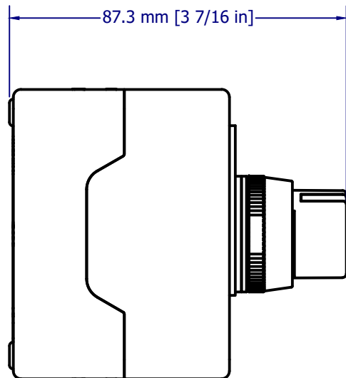
Single hole assembly w/selector switch
