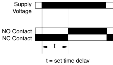
FUNCTION: ON DELAY
