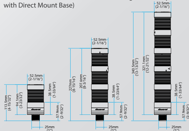
Series WTL-50P3 (50mm Diameter Tower Light Assembly with Direct Mount Base)
