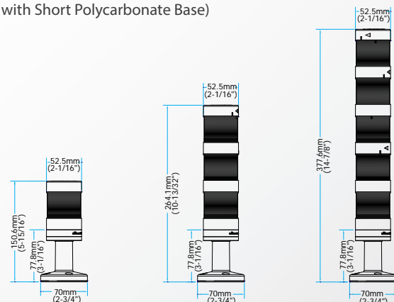
Series WTL-50P2 (50mm Diameter Tower Light Assembly with Tall Polycarbonate Base)
