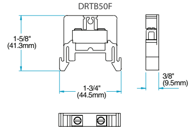
50A Feed Through Terminal Block (Box Type)
