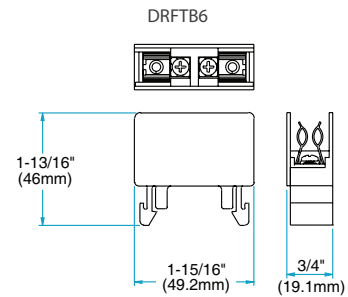
NEMA Fusible Terminal Block
