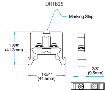
25A Feed Through Terminal Block (Modular)
