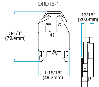
NEMA Fusible Terminal Block
