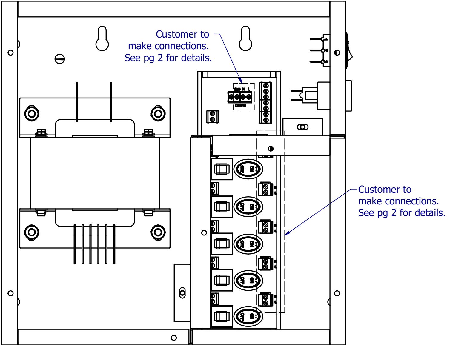
VIEW1 - Enclosure With Covers Off SCALE 1/2
