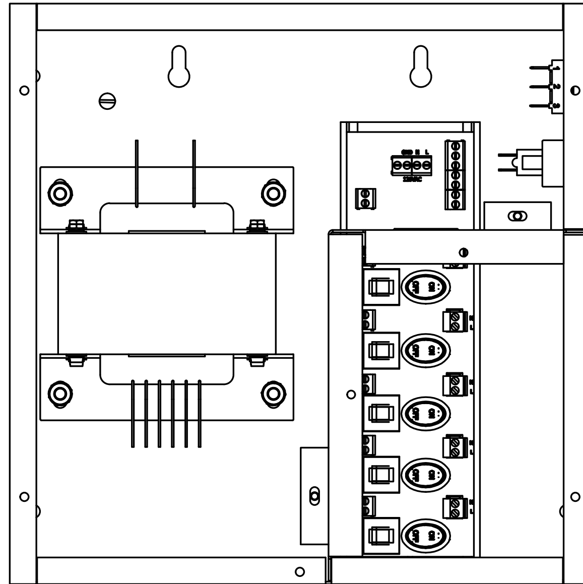
Front View (Cover Off) SCALE 1/2
