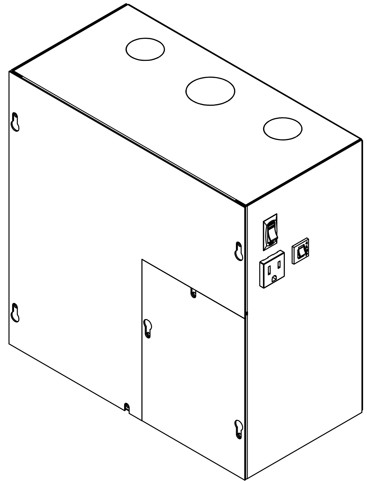
Isometric View SCALE 1/2
