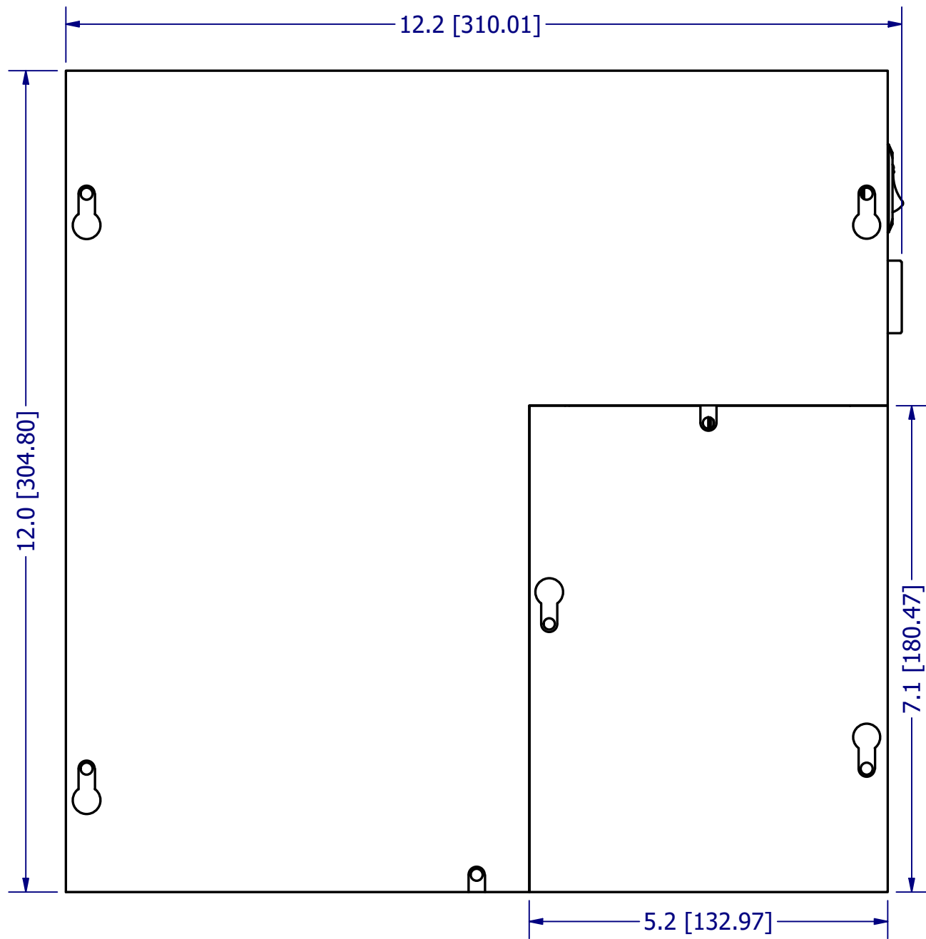
Front View SCALE 1/2
