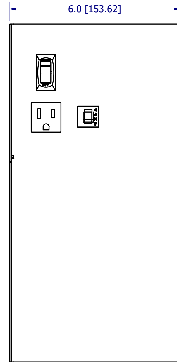
Side View SCALE 1/2
