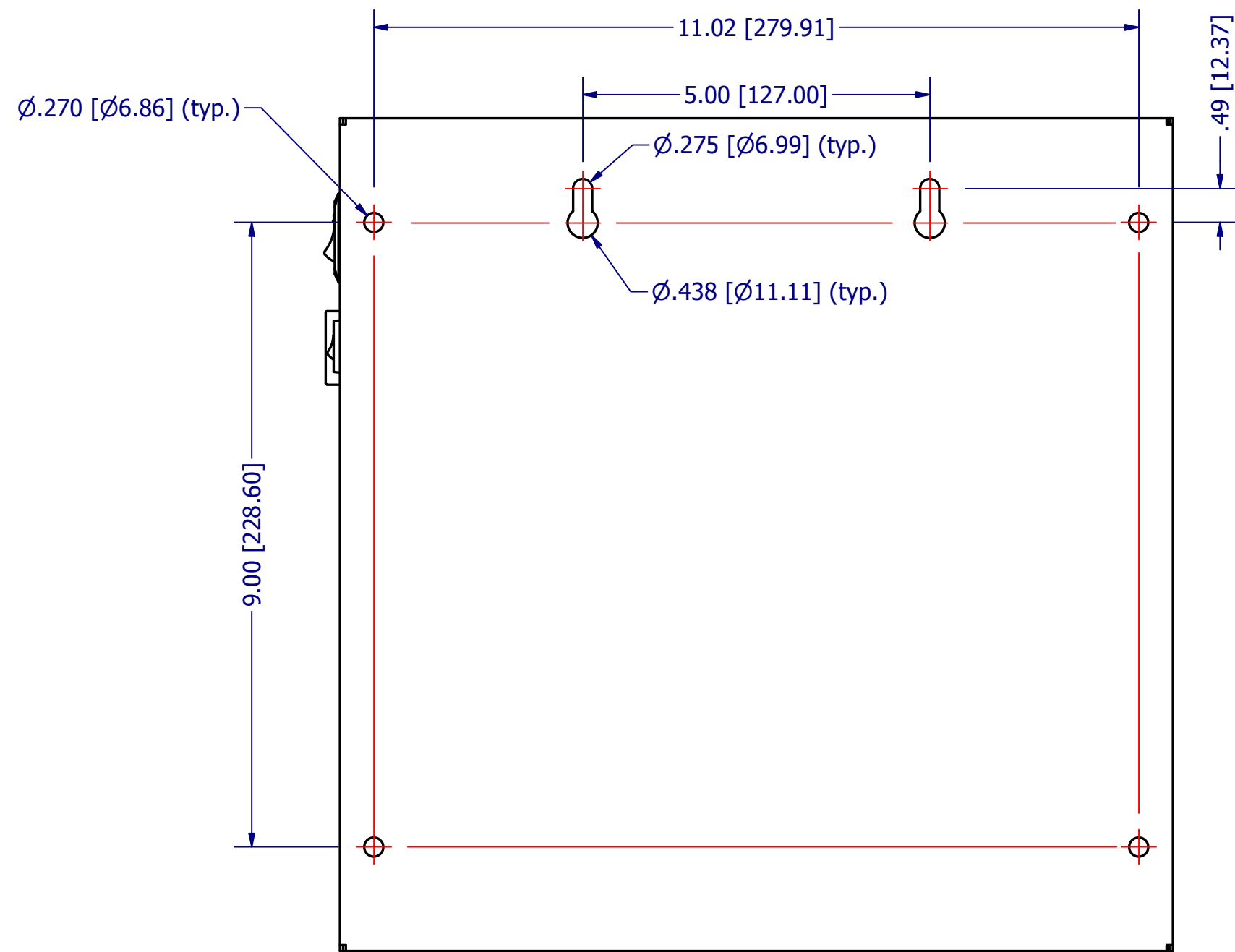
Back View SCALE 1/2
