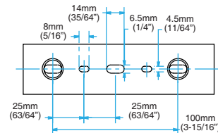
DUCT WIDTH: 40mm and 60mm
