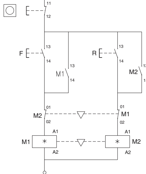
CONTROL CIRCUIT
