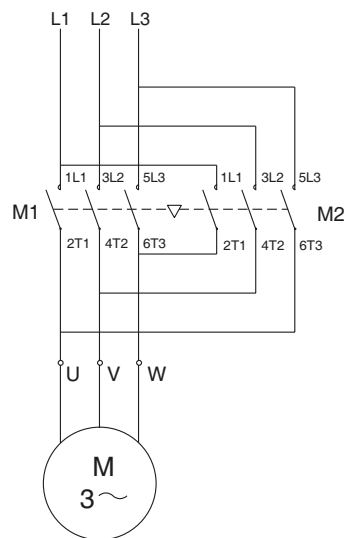
POWER CIRCUIT
