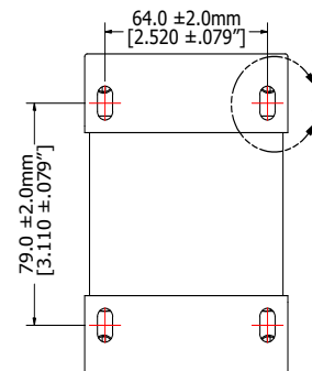
MOUNTING DIMENSIONS
