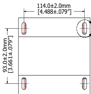
MOUNTING DIMENSIONS
