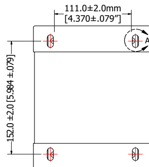
MOUNTING DIMENSIONS
