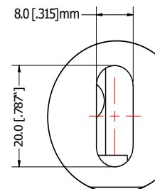
DETAIL A
