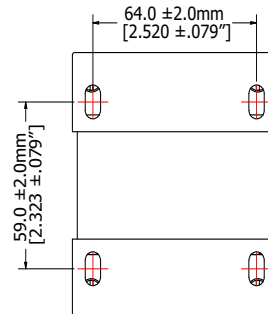
MOUNTING DIMENSIONS
