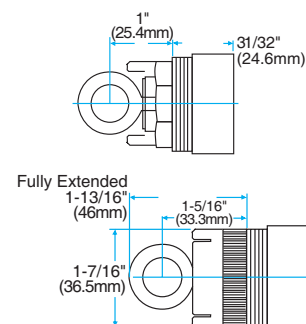
MOMENTARY AND HEAVY DUTY CABLE PULL OPERATORS
