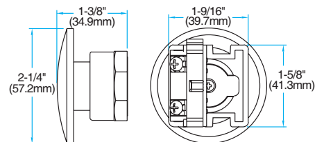
MOMENTARY 2-1/4" (57.2MM) JUMBO MUSHROOM CAP
