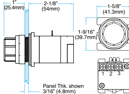
POTENTIOMETER OPERATOR (SHOWN WITH TERMINAL BLOCK)
