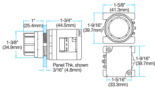
POTENTIOMETER OPERATOR (SHOWN WITHOUT TERMINAL BLOCK)
