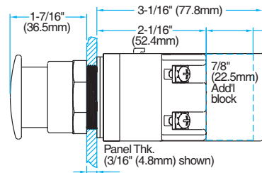
ILLUMINATED RESISTOR OPERATOR (SHOWN WITH IMC)
