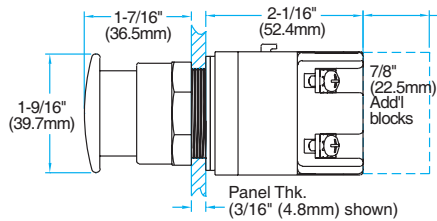
ILLUMINATED FULL VOLTAGE OPERATOR (SHOWN WITH IMC)
