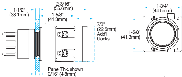
ILLUMINATED SHROUDED MUSHROOM LENS (SIPBCM)
