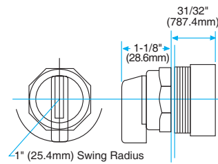
SELECTOR SWITCH LEVER HANDLE
