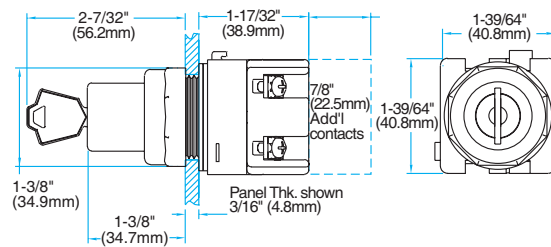
KEYED SELECTOR SWITCH OPERATOR
