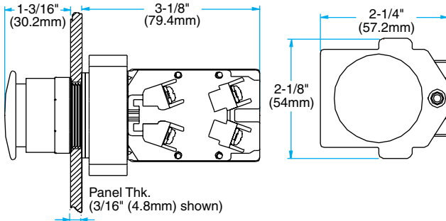
FULL VOLTAGE PUSH-TO-TEST OPERATOR (SHOWN WITH HIPBCM)
