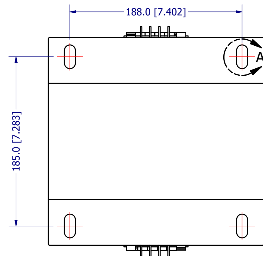
MOUNTING DIMENSION
