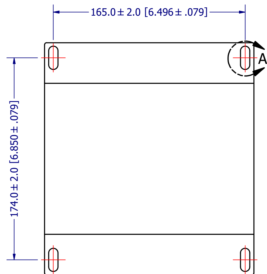
MOUNTING DIMENSION
