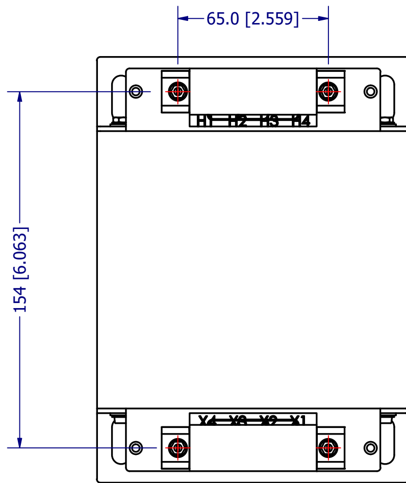
TOP VIEW
