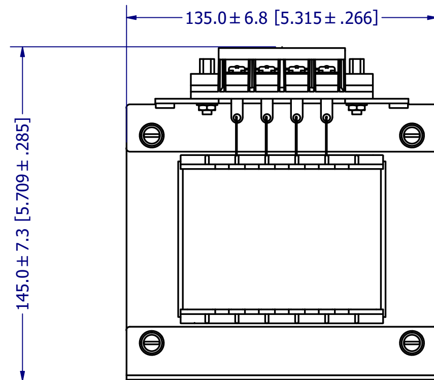
FRONT VIEW
