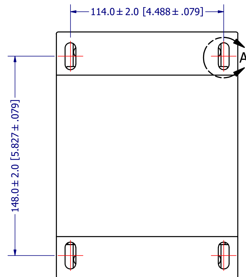
MOUNTING DIMENSION
