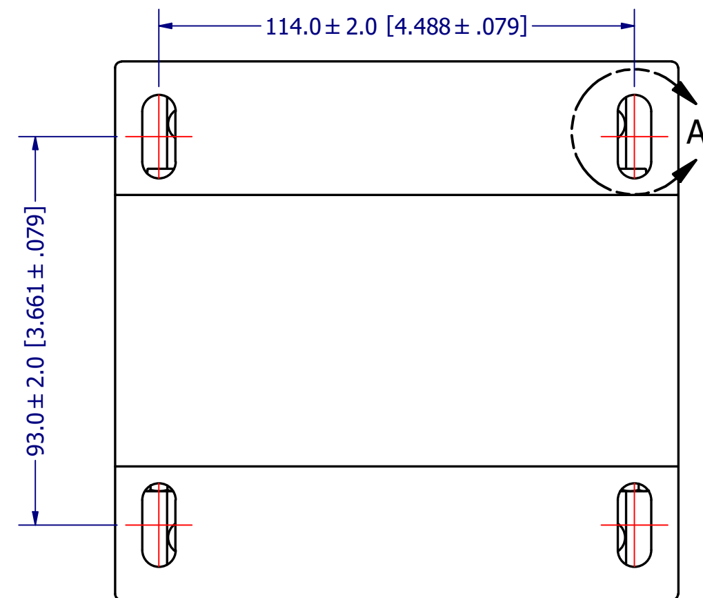
MOUNTING DIMENSION
