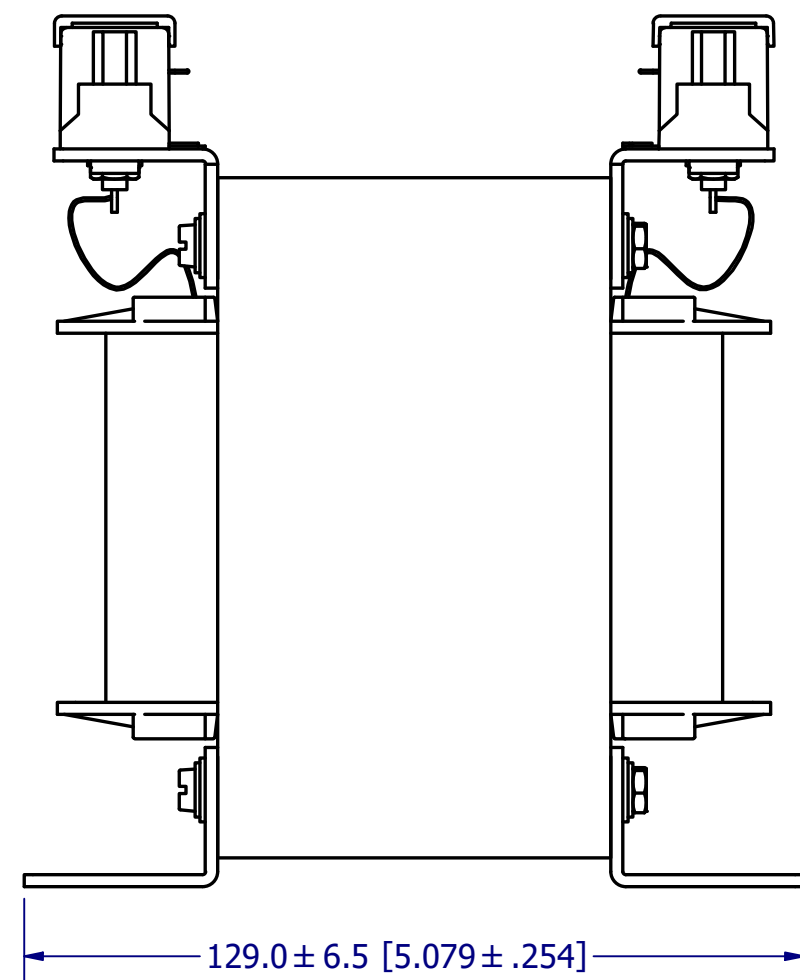
SIDE VIEW
