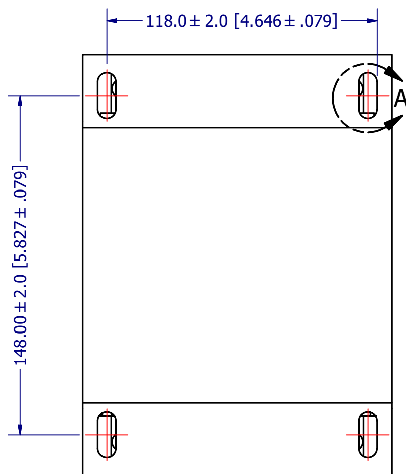
MOUNTING DIMENSION
