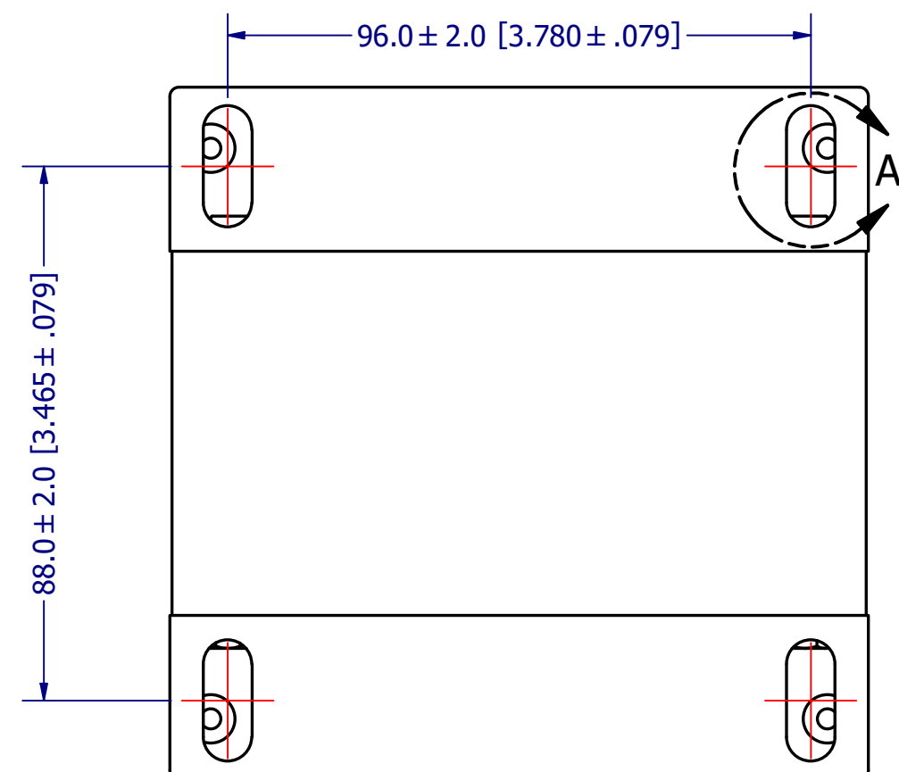
MOUNTING DIMENSION
