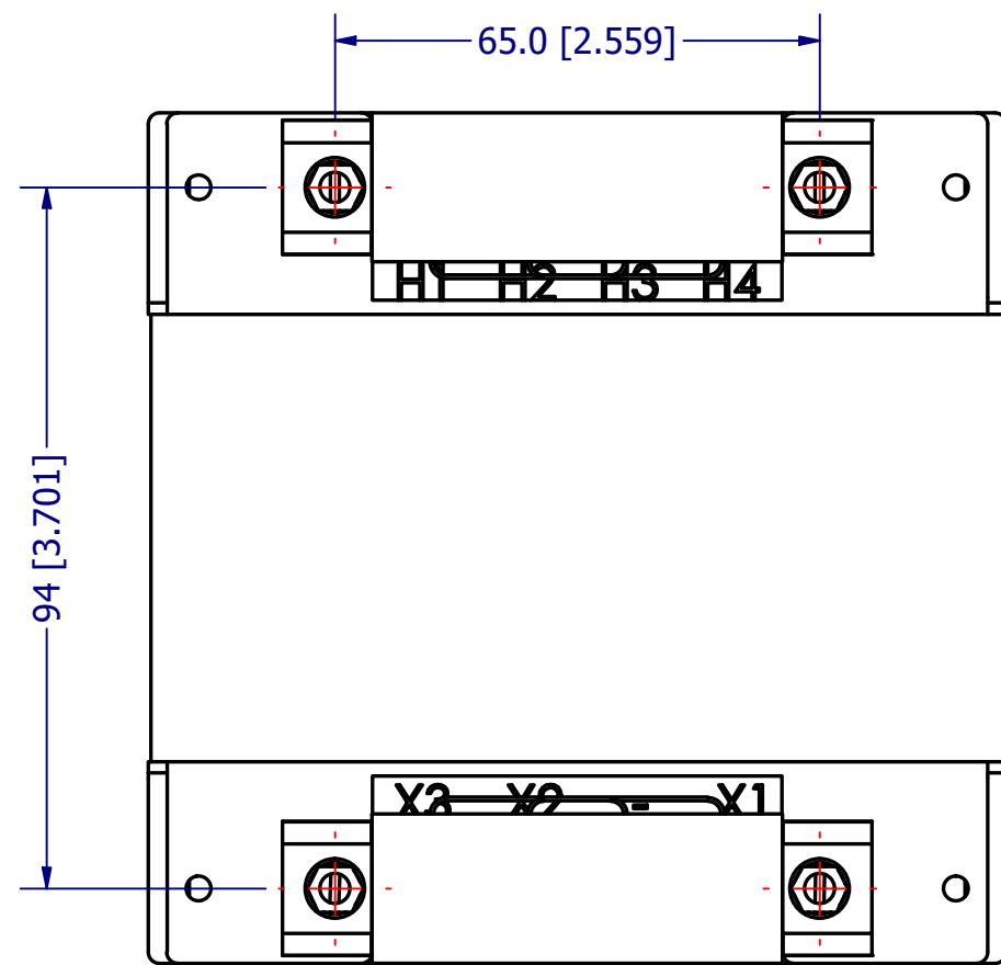
TOP VIEW
