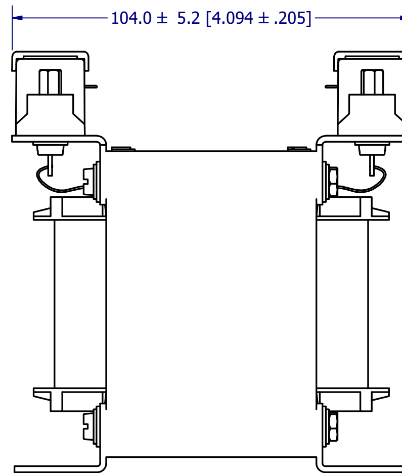
SIDE VIEW
