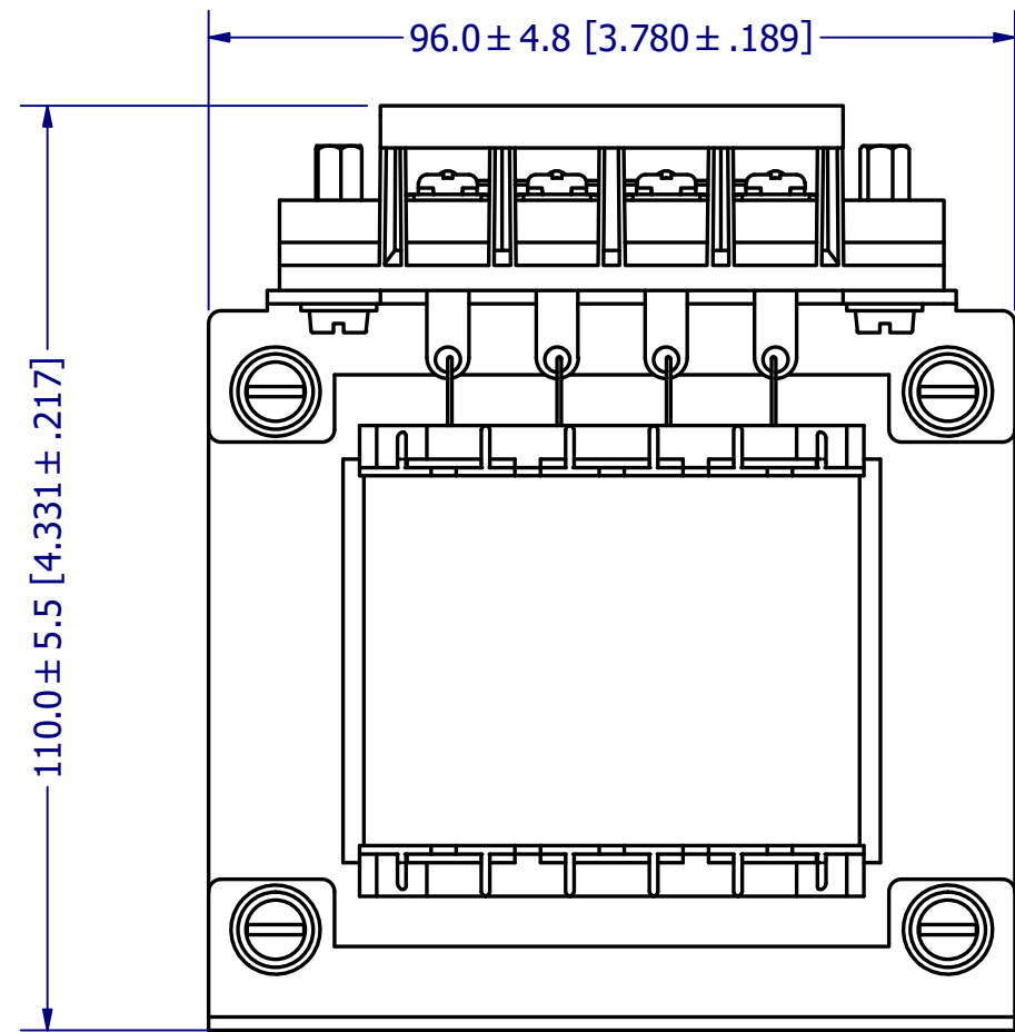
FRONT VIEW
