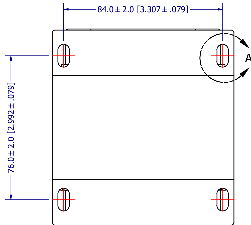
MOUNTING DIMENSION
