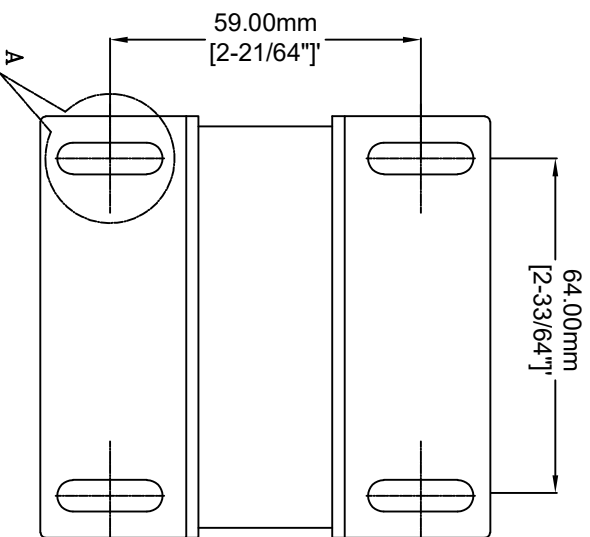
MOUNTING DIMENSIONS
