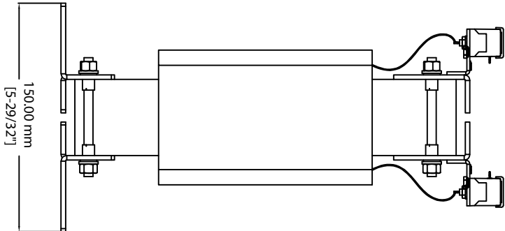
SIDE VIEW
