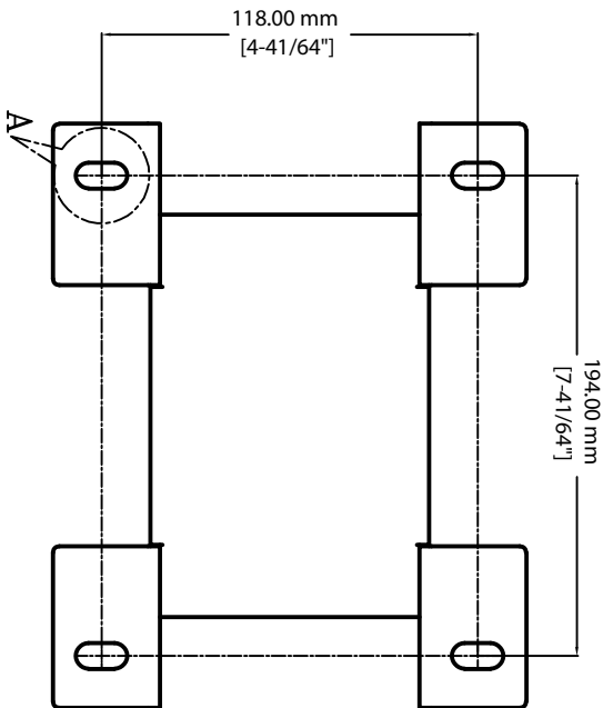
MOUNTING DIMENSIONS
