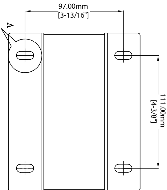
MOUNTING DIMENSIONS
