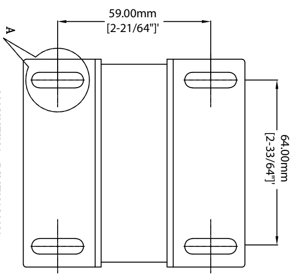
MOUNTING DIMENSIONS
