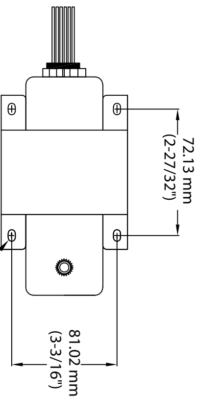
TOP VIEW
