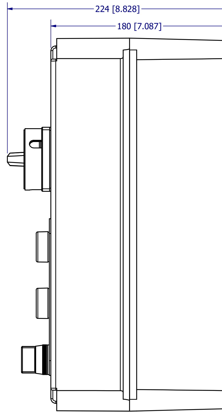
Side View SCALE 1/2
