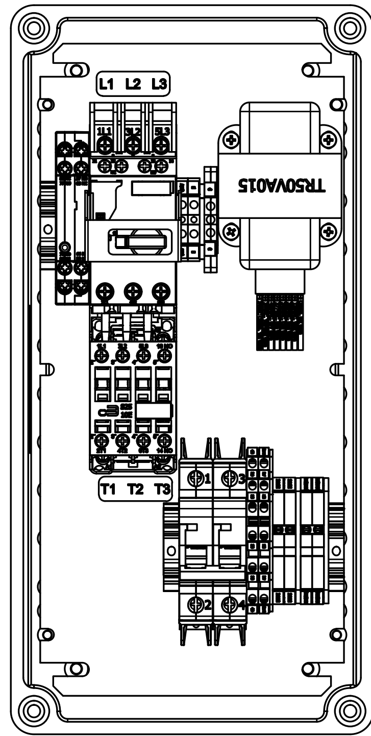
Cover Off SCALE 1/2
