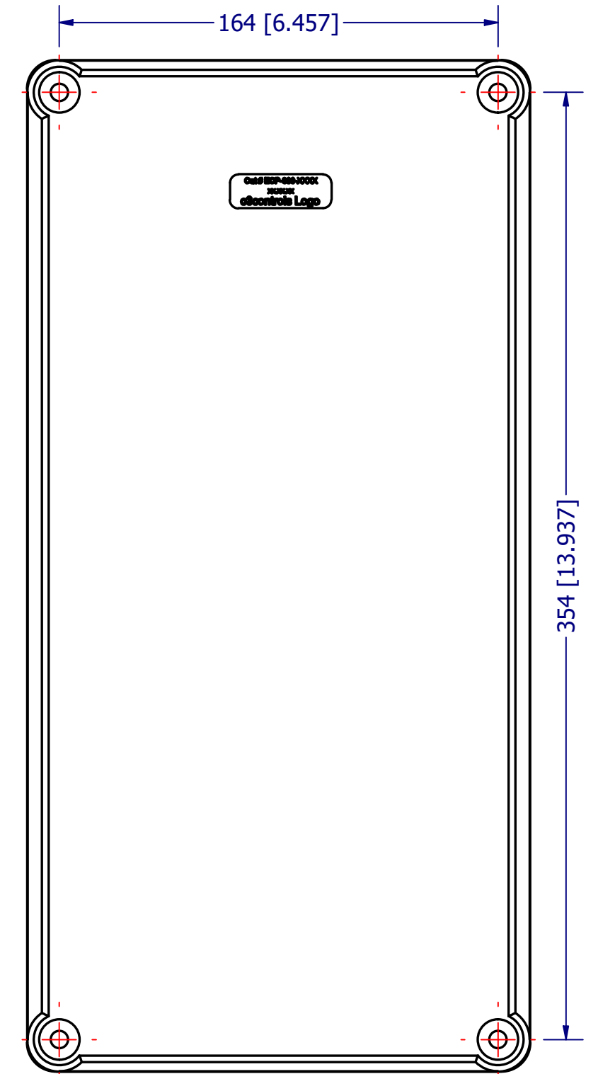
Back View SCALE 1/2
