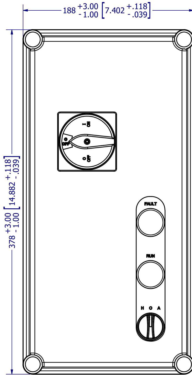
Front View SCALE 1/2
