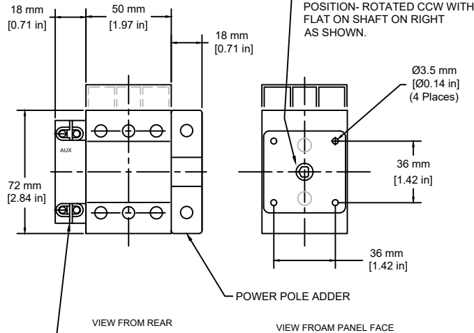
AUXILIARY CONTACTS
